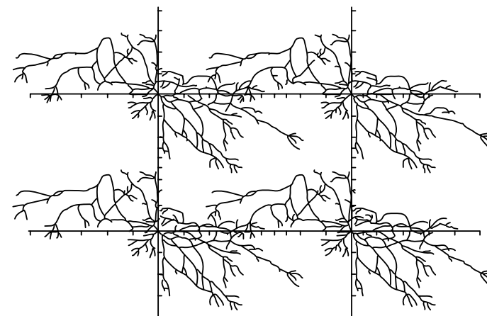
Figure 2. Root systems of adjacent trees add reinforcement strength as they mesh together.
